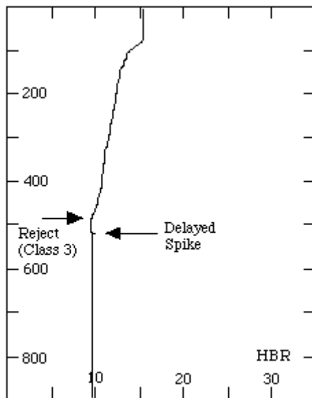
Figure 3.1R Hit Bottom Reject (HBR)
