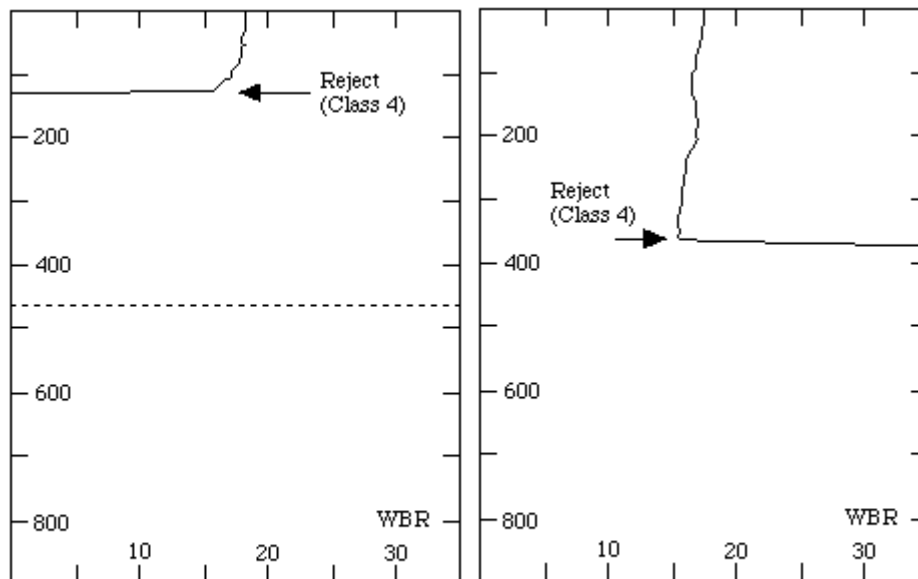
Figure 3.2R.1 Wire Break Reject From Launcher Spool (WBR)
