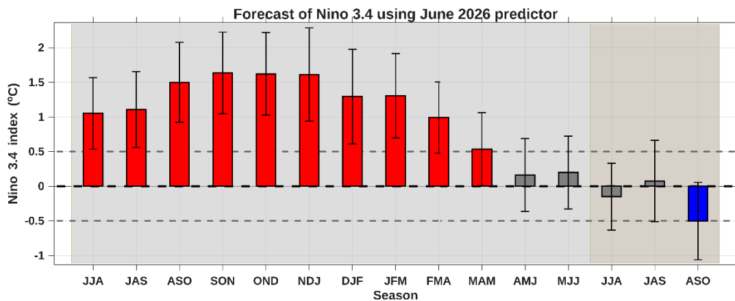
Fig. 4: Median prediction of Nino 3.4 index using April 2026 - June 2026 predictors for the upcoming seasons.
