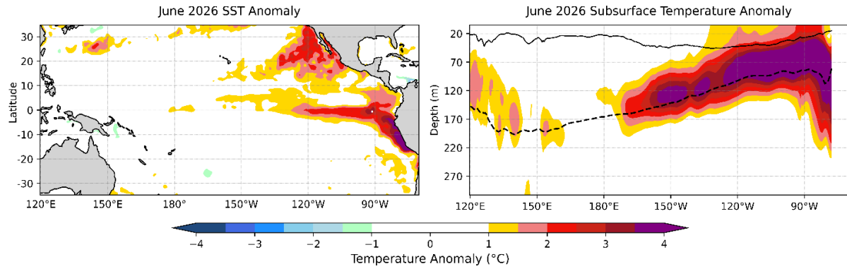
Fig. 3: (Left) Monthly SST anomaly for the tropical Pacific in June 2026. (Right) Subsurface temperature anomaly averaged over 5° S-5° N for June 2026.
