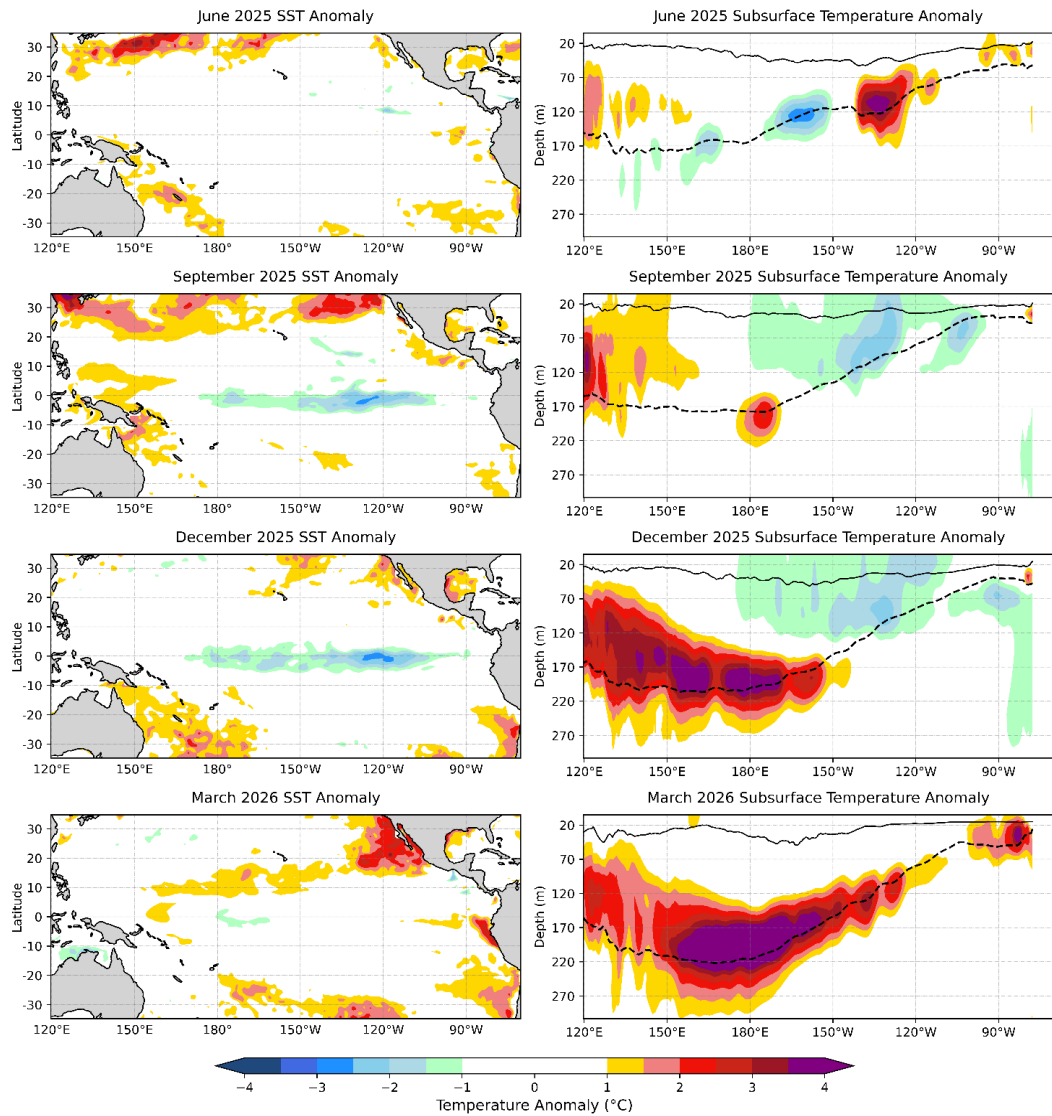
Fig. 2: (left) Monthly SST anomaly for the tropical Pacific. (Right) Subsurface temperature anomaly averaged over 5^{\circ}\text{S} - 5^{\circ}\text{N} for the corresponding months.
