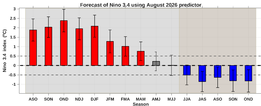
Fig. 4: Median prediction of Nino 3.4 index using June 2026 - August 2026 predictors for the upcoming seasons.
