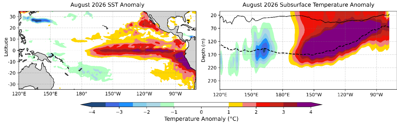
Fig. 3: (Left) Monthly SST anomaly for the tropical Pacific in August 2026. (Right) Subsurface temperature anomaly averaged over 5° S-5° N for August 2026.
