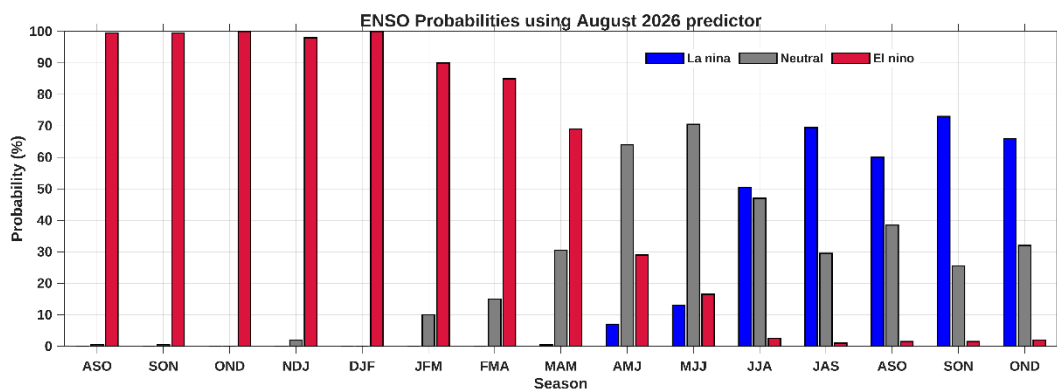
Fig. 5. Forecast of El Niño/La Niña conditions using June 2026 - August 2026 predictors.
