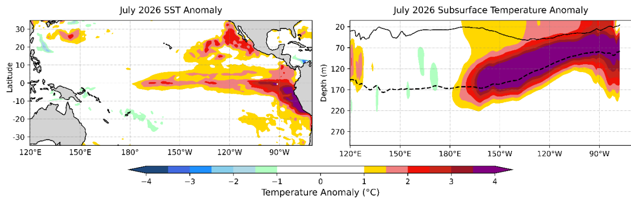
Fig. 3: (Left) Monthly SST anomaly for the tropical Pacific in July 2026. (Right) Subsurface temperature anomaly averaged over 5° S-5° N for July 2026.
