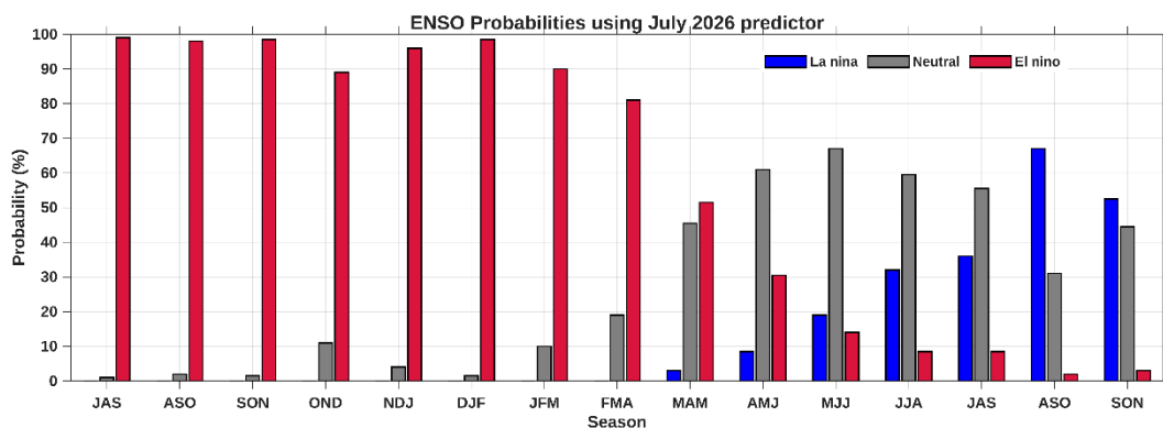
Fig. 5. Forecast of El Nino/La Nina conditions using May 2026 - July 2026 predictors.
