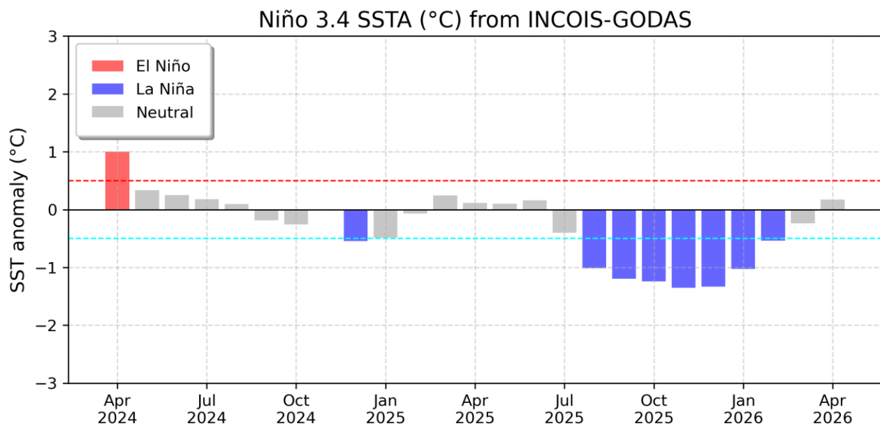
Fig. 1: Evolution of Sea Surface Temperature anomalies (°C) in the Niño 3.4 (5°S-5°N, 170°W-120°W) region in the period April 2024 - April 2026. The RED and CYAN horizontal lines represent 0.5°C SST anomaly
